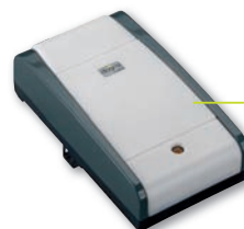
Proton
